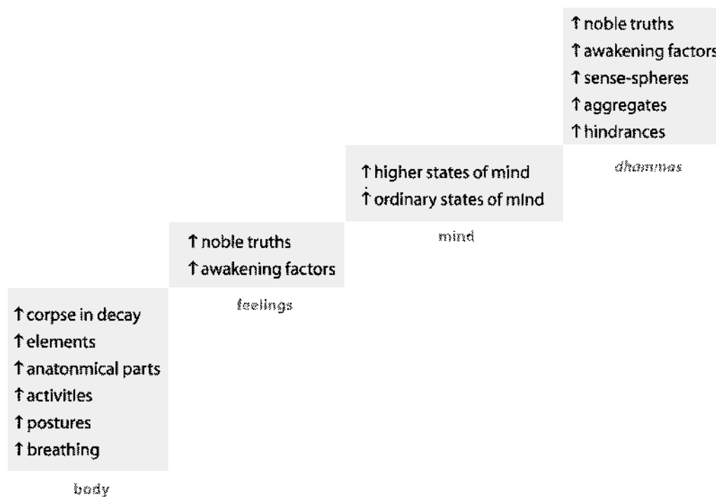
Fig. 1.2 Progression of the Satipaṭṭhāna contemplations
